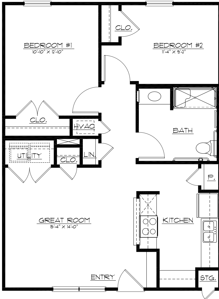
TWO BEDROOM, ONE BATH UNIT (H.C.) 794 S.F.
